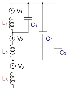
Fig. 6. A circuit diagram for a triply-tuned MACS resonator. V_1 , V_2 , and V_3 represent electromotive forces induced by the primary circuit in the probe.
