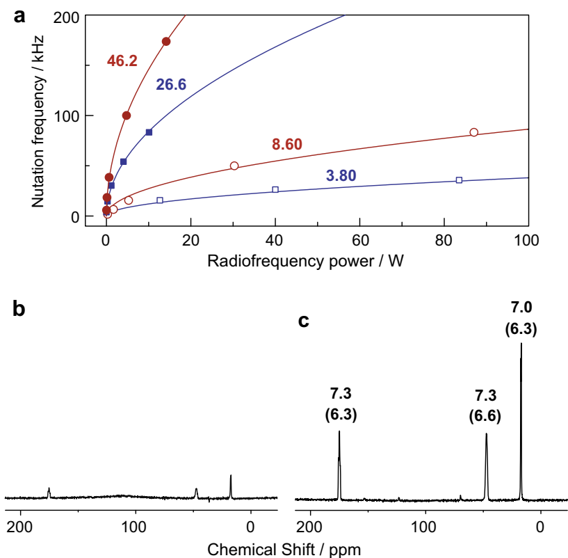
Fig. 3. (a) Radiofrequency-power dependence of the nutation frequencies for the ^{13}\text{C} and ^1\text{H} spins in a Varian 5 mm CP-MAS probe at 75 and 300 MHz. The magnetic field was 7 T. The blue symbols represent the ^{13}\text{C} nutation frequencies with (filled squares) and without (open squares) the doubly-tuned MACS resonator, and the red symbols represent the ^1\text{H} nutation frequencies with (filled circles) and without (open circles) the MACS resonator. The data points were fitted by a square root function of the form y = a\sqrt{x} , and the coefficient a is depicted for each set of the data. (b) A ^{13}\text{C} CP-MAS spectrum of polycrystalline ^{13}\text{C} - ^{15}\text{N} -labeled L-alanine obtained without the doubly-tuned MACS resonator. The sample ( \sim 0.1 mg) was packed in a capillary tube and put into the rotor using a spacer. (c) A ^{13}\text{C} spectrum of the identical sample obtained by employing the doubly-tuned MACS resonator. The numbers 7.0, 7.3, and 7.3 indicate the enhancement factors of the ^{13}\text{C} peak intensities for the methyl, methine, and carboxyl carbon sites in L-alanine, while the numbers in the parentheses are the overall enhancement factors in the signal-to-noise ratio by taking account of the additional noise arising from the MACS insert. In both (b) and (c), the spinning frequency was 8 kHz, and the signals were accumulated over 1000 times under TPPM ^1\text{H} decoupling with an intensity of 100 kHz.
