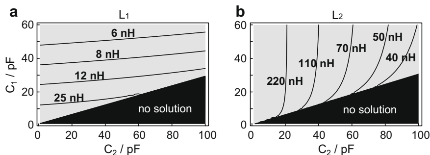
Fig. 2. The contour plots in (a) and (b) describe the L_1 and L_2 values required to tune the circuit at both 300 and 75 MHz for a given set of the capacitances C_1 and C_2 . These plots are calculated from Eqs. (2)–(5), and in the present work, L_1 = 11 nH, L_2 = 43 nH, C_1 = 33 pF, and C_2 = 82 pF.
