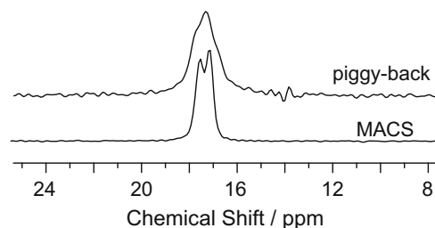
Fig. 5. Comparison of the resonance line width of the methyl ^{13}\text{C} in a polycrystalline sample of ^{13}\text{C} - ^{15}\text{N} -labeled L-alanine for the MACS and piggy-back schemes under TPPM ^1\text{H} decoupling with an intensity of 100 kHz. The spinning frequency was 8 kHz.
