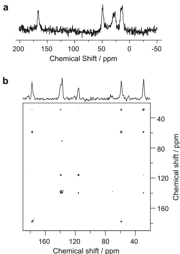
Fig. 4. (a) A ^{13}\text{C} CP-MAS spectrum of A \beta 42 ( \sim 0.1 mg of sample) partially ^{13}\text{C} -labeled at the 35-Met and 42-Ala amino acid residues. The sample was synthesized as reported previously [16]. The ^{13}\text{C} NMR signals were accumulated over 180,000 times with a recycle delay of 1 s. The spinning frequency was 10 kHz. (b) A two-dimensional ^{13}\text{C} - ^{13}\text{C} DARR correlation spectrum in uniformly ^{13}\text{C} -labeled polycrystalline histidine ( \sim 0.1 mg of sample). 128 hypercomplex data points were acquired in the indirect dimension, and each of them was accumulated over 1280 times with a recycle delay of 0.5 s. The spinning frequency was 5 kHz. Both data were acquired using the doubly-tuned MACS resonator.
